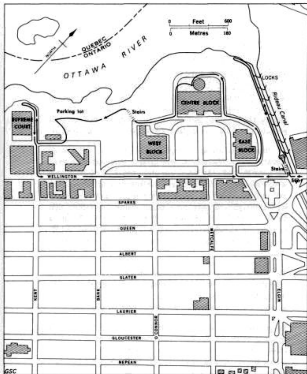
Trip 1. Rideau Canal and Parliament Buildings
