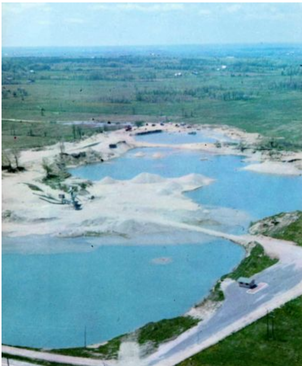
Blue-green, lime-rich waters fill partly abandoned quarries west of Aylmer.
