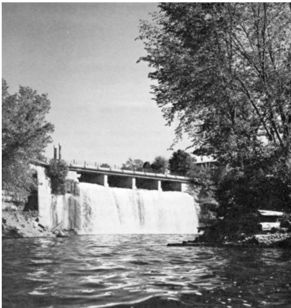
The smaller of the two Rideau Falls on the west side of Green Island.
