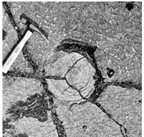
Large algal head weathering out of limestone above the Orleans quarry, east of Ottawa.
