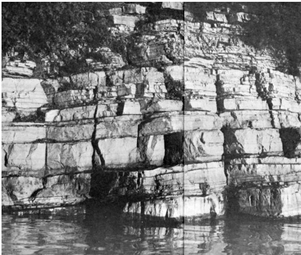
Bedding and jointing in the Ottawa limestone just below the Prime Minister's residence on the Ottawa River.
