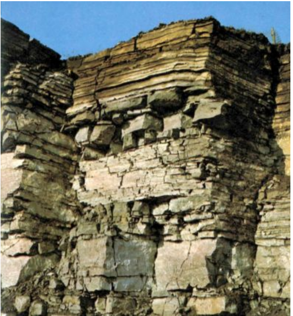
Jointed limestone of the Hull member of the Ottawa Formation shows weather staining near the old surface, in a road-cut just west of the Canada Cement plant quarry in Hull.
