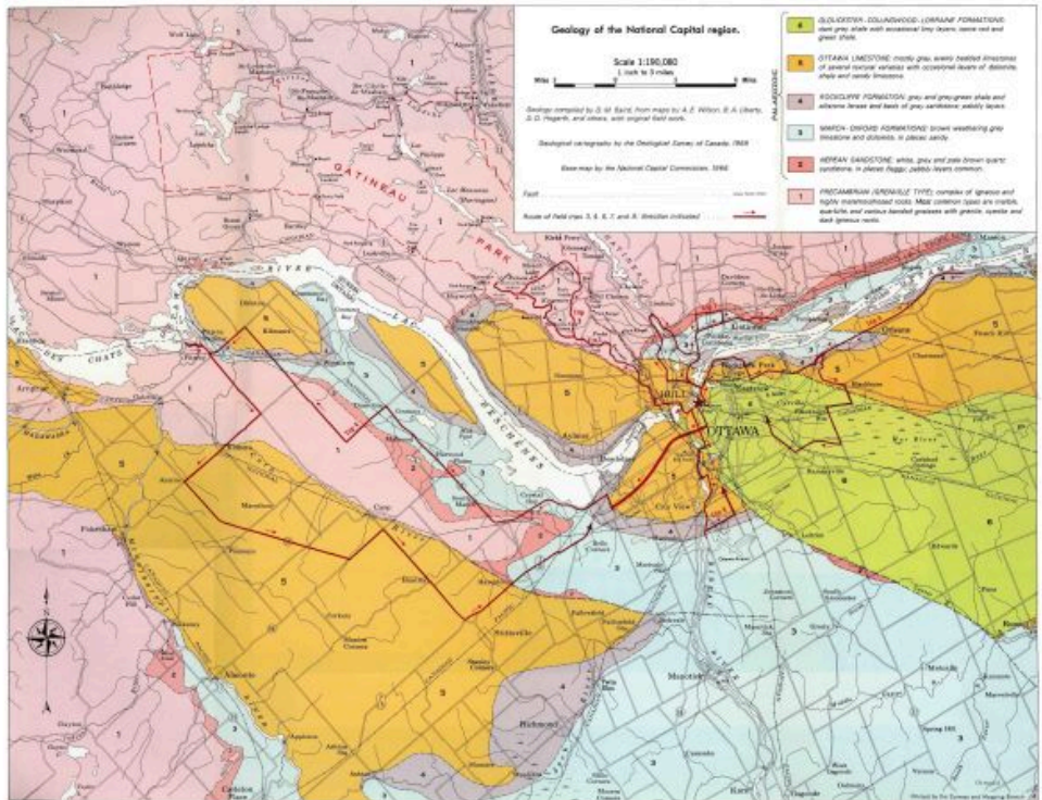
Geology of the National Capital region.
