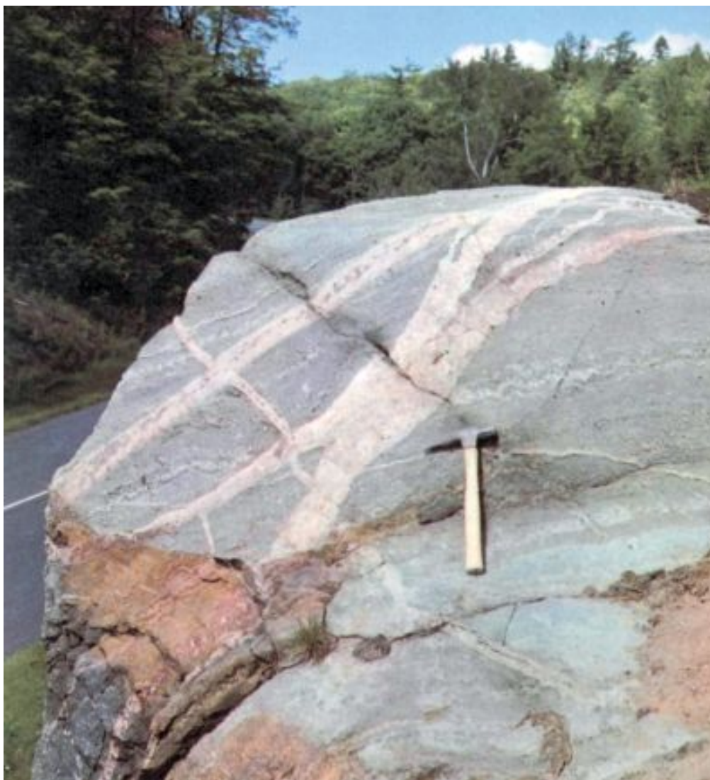
Criss-crossing pink aplite dykes cut older gneisses beside the Gatineau Parkway.
