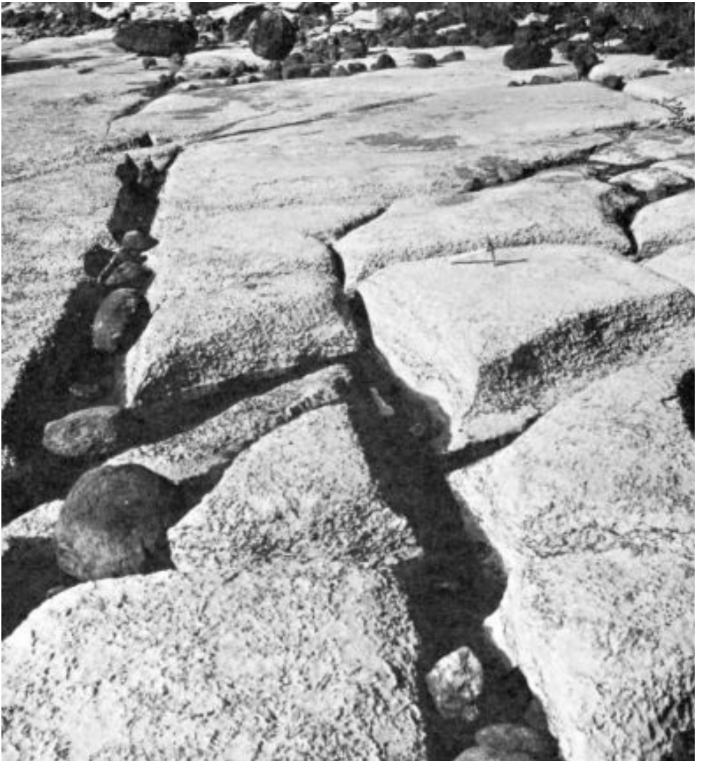
An outcrop of very white Ottawa limestone in the Ottawa River bed dissolves slowly away, leaving the more-resistant matter standing up in relief. The dark, manganese-stained boulders contrast with the white limestone. This is seen at Alumette Rapids, west of the National Capital area.
