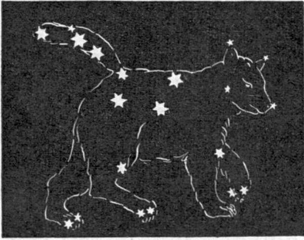
THE GROUP OF STARS THAT MAKE UP THE GREAT BEAR
