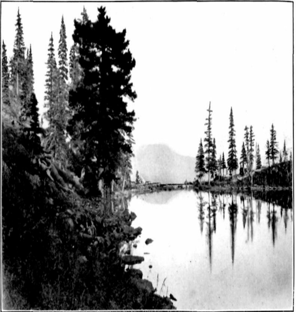
LAKE AGNES, A GOOD EXAMPLE OF A CIRQUE LAKE
