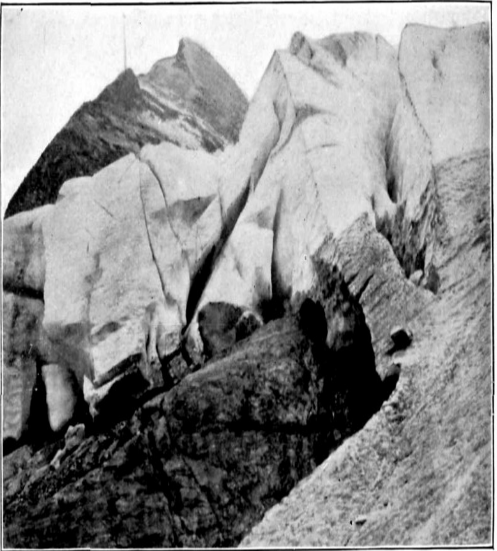
ICE BRIDGE ON ILLECILLEWAET GLACIER
