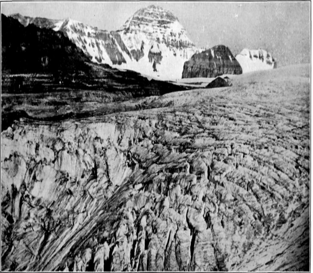
CREVASSES, GLACIER SOUTHEAST OF TEN PEAKS
