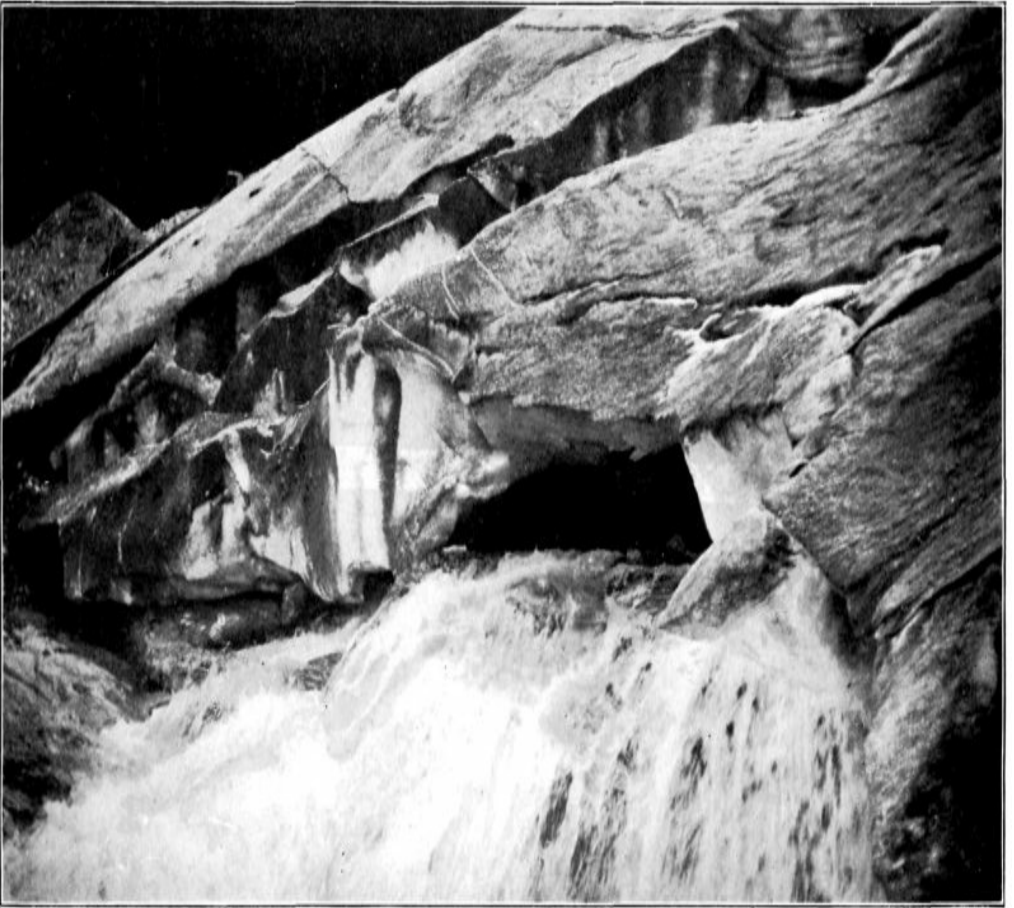
GLACIAL STREAM, MT. ROBSON, DIVIDING ITS WATERS BETWEEN THE PACIFIC AND ARCTIC OCEANS
