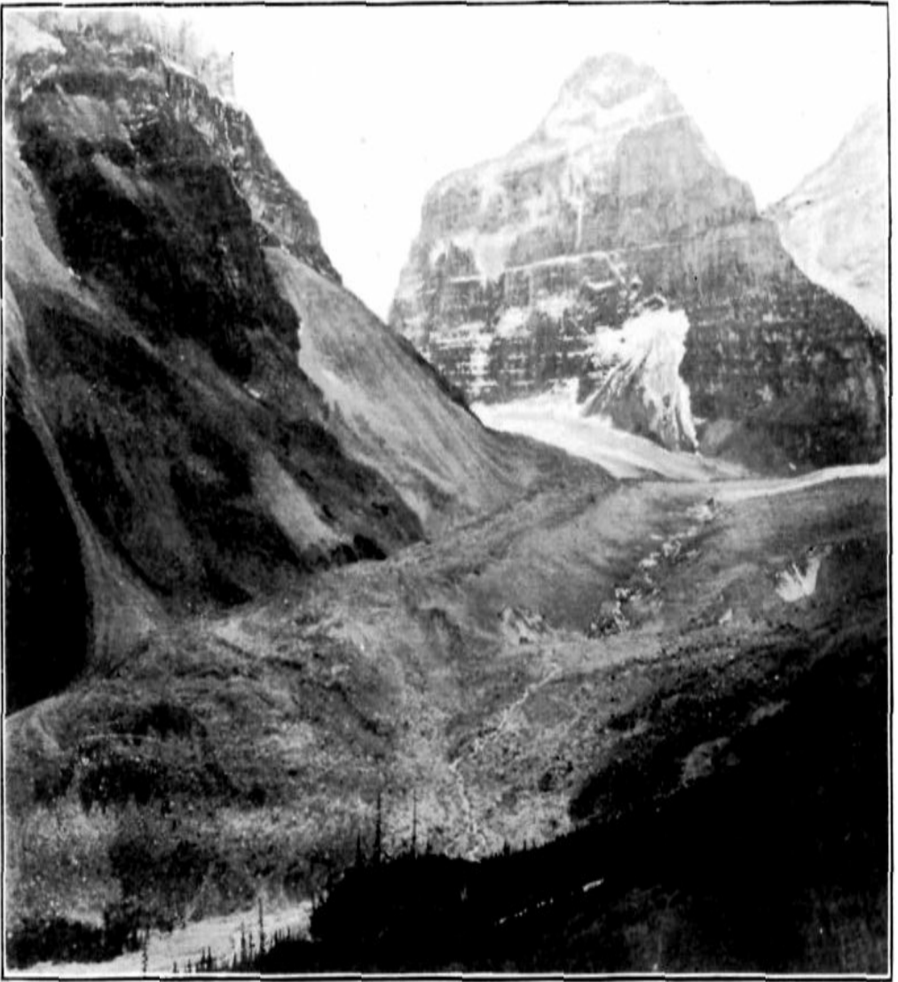
MORAINE OF VICTORIA GLACIER
