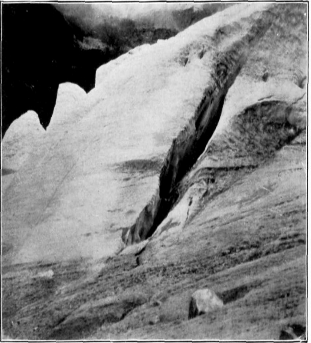
CREVASSE ON GREAT GLACIER
