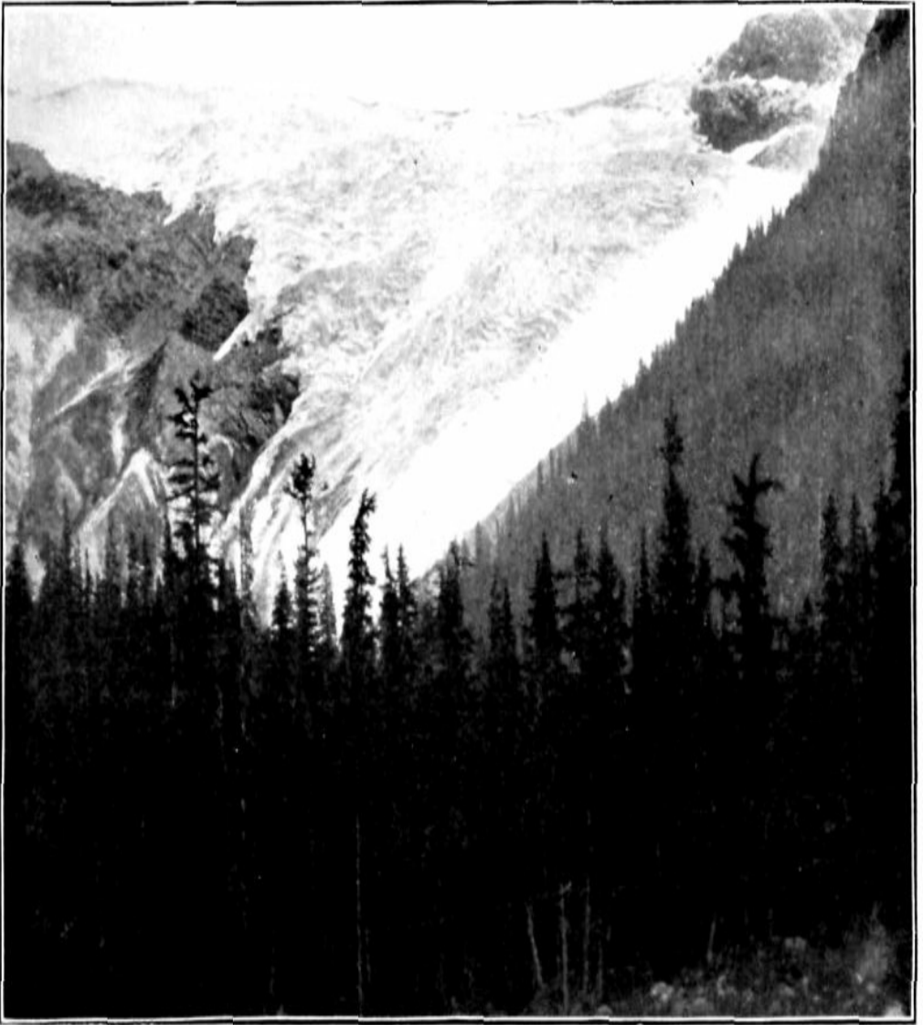
THE ILLECILLEWAET OR GREAT GLACIER, GLACIER PARK
