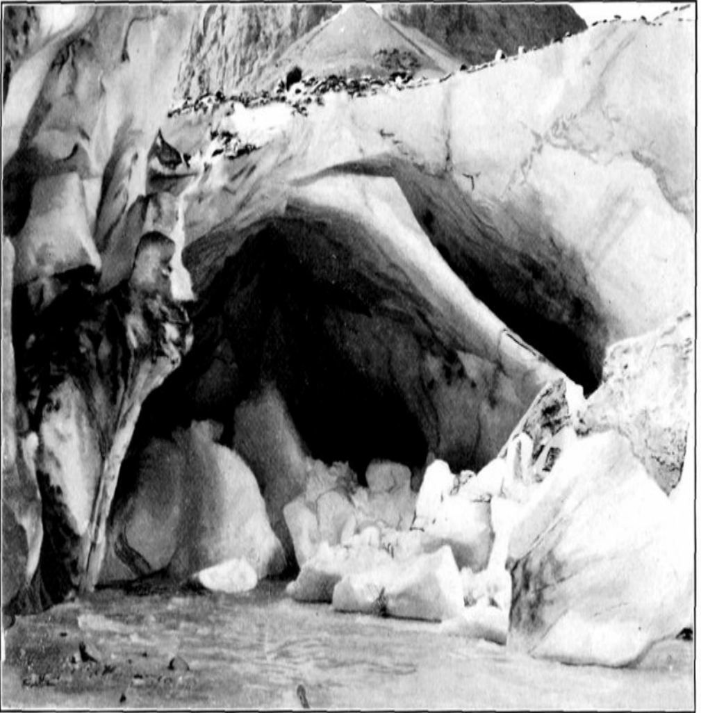
SNOUT OR FOREFOOT OF ROBSON GLACIER, JASPER PARK
