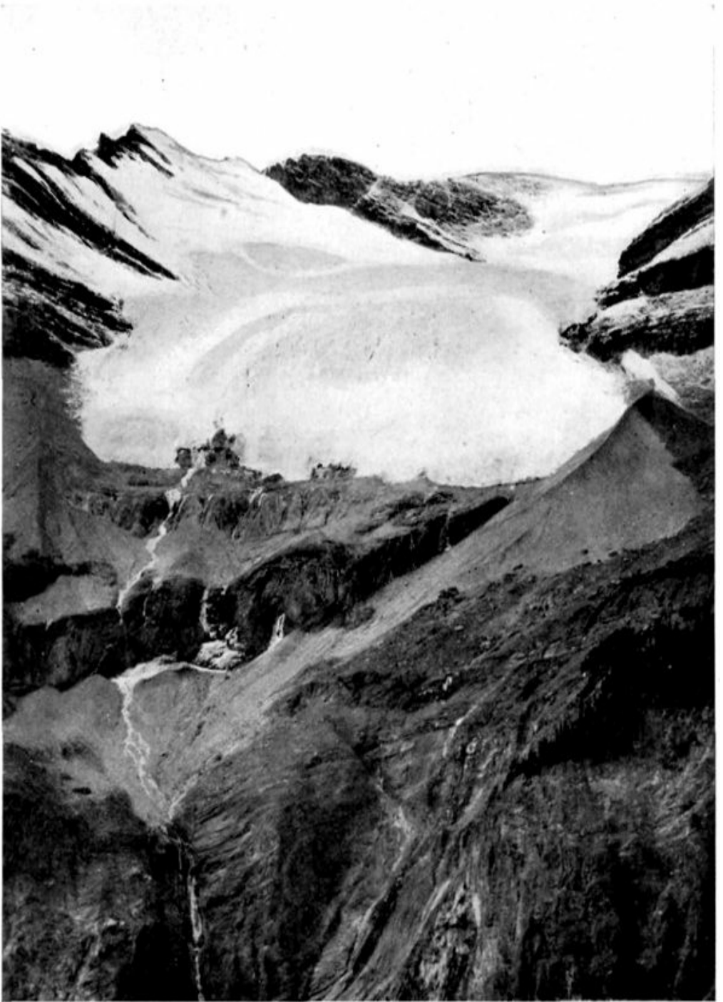
GLACIER ON PRESIDENT RANGE, YOHO PARK
