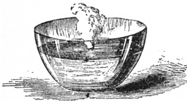
Fig. 1.—Piece of potassium in a basin of water.
