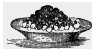
Fig. 41.— Carbon rising up from white sugar.
