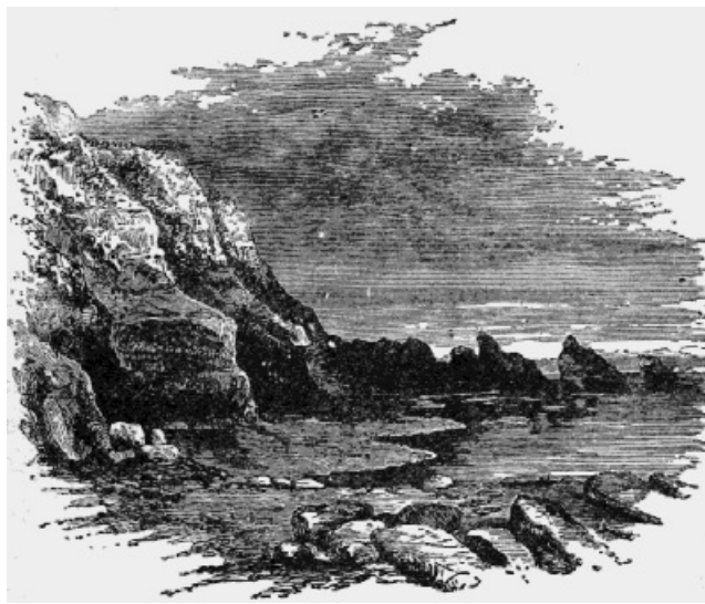
Fig. 28.—Cliffs off Arbroath, showing the waste of the shore.
