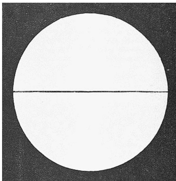
Fig. 4.—106 earths laid across the face of the sun. Each one of these dots represents roughly the size of the earth as compared to the size of the sun represented by the large circle.
