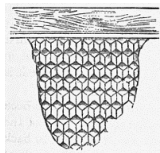
Fig. 55.—Plate of wax with bases of cells, hanging from the bar of a hive.
