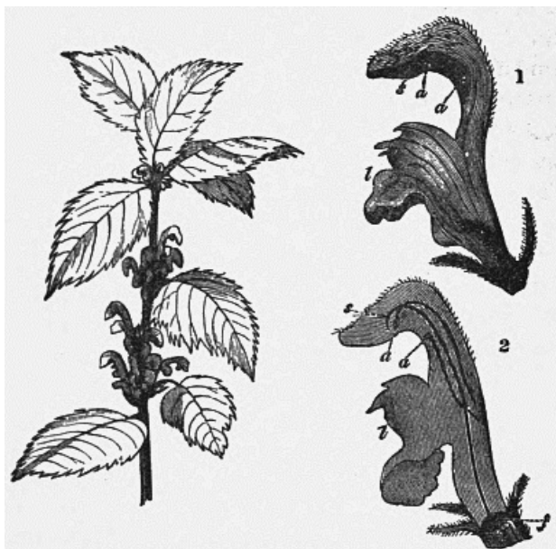
Fig. 59.—Flower of the Dead-Nettle ( Lamium album ).
