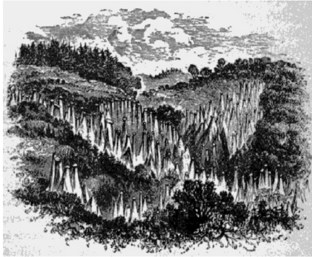
Fig. 24.—Earth-pillars near Botzen, in the Tyrol. (Adapted from Lyell's 'Principles.')
