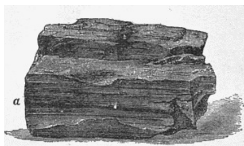
Fig. 45.—Piece of coal. a, Smooth face, showing laminæ or thin layers.
