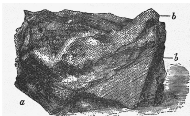
Fig. 47.—A piece of shale with impressions of ferns and Calamite stems.
