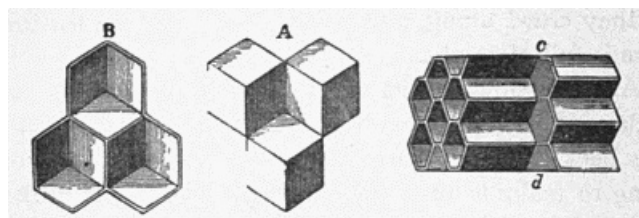
Fig. 56.—B shows in the centre the closed end of a cell which would fit into the space in the centre of the three closed cells in A, while the ends of these three would fit into the spaces in B. B. c, d, side-view of cells.
