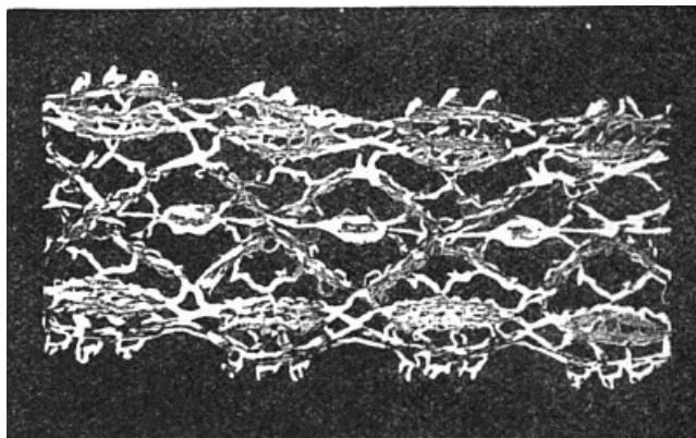
Fig. 9. —Piece of lace photographed during the lecture.
